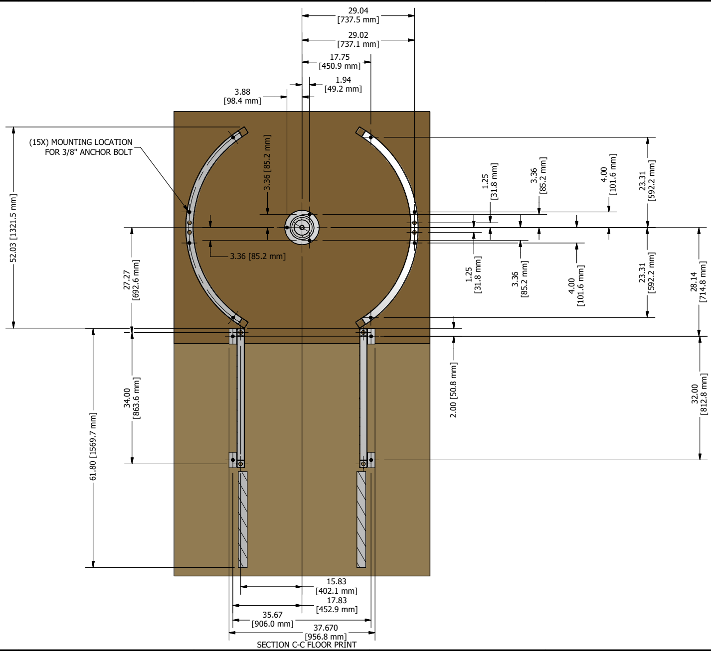
SECTION C-C FLOOR PRINT
