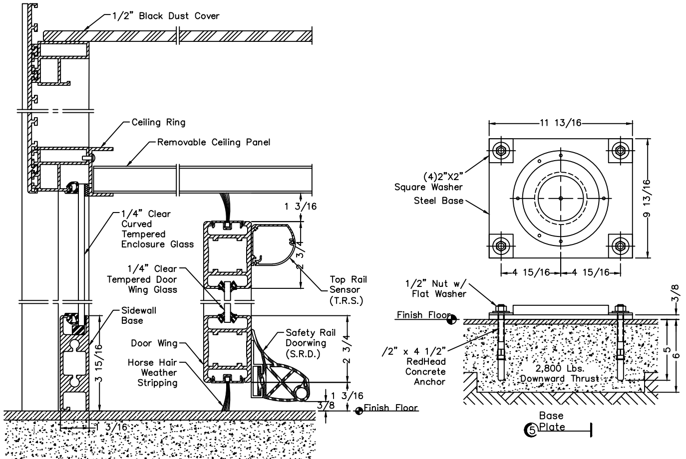
3 Vertical Sections
