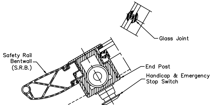
Horizontal Sections
