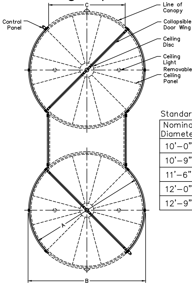
② Plan View
