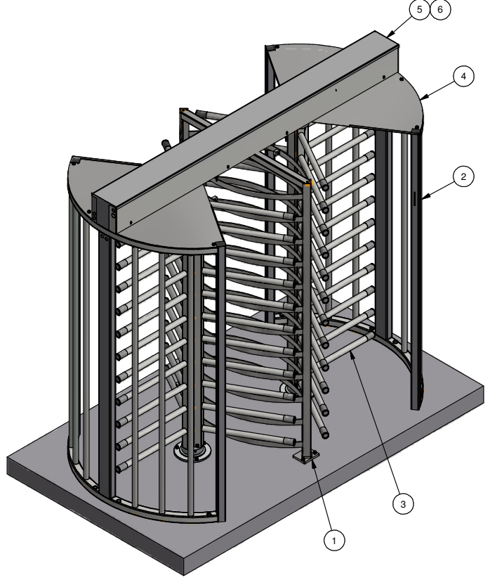
ISOMETRIC SCALE 1:21
