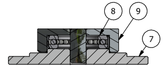
SECTION A-A BOTTOM BEARING/BASE PLATE SCALE 1:4
