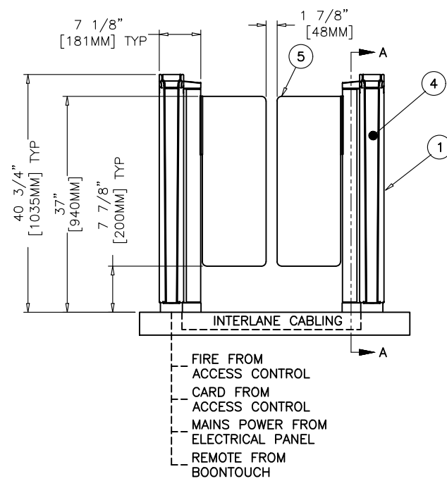
② ELEVATION VIEW
