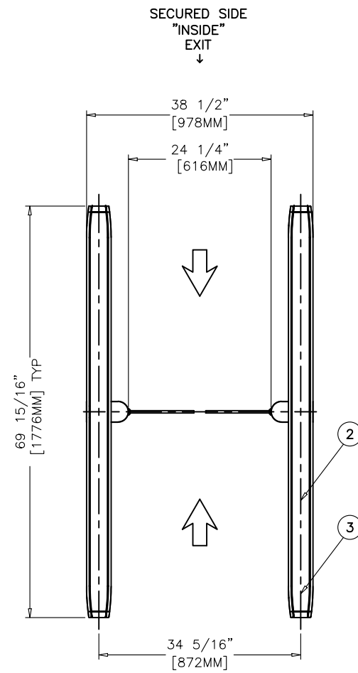
NON-SECURED SIDE "OUTSIDE" ENTRY ↑ ① PLAN VIEW
